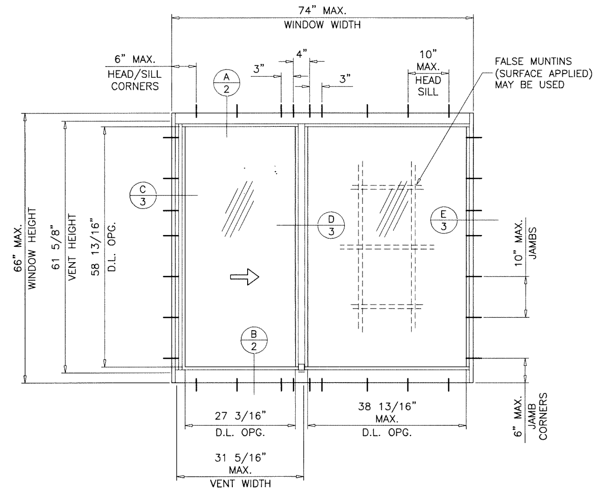
TYPICAL ELEVATION
